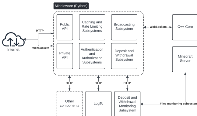
Fig. 6. Middleware
